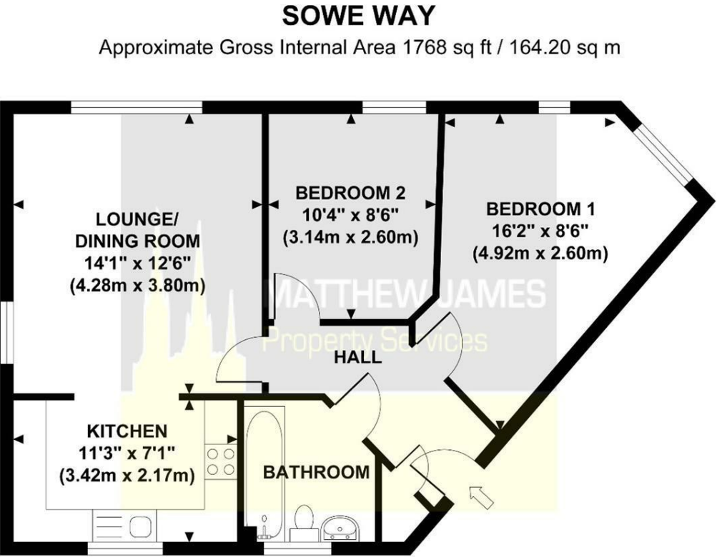
GROSS INTERNAL FLOOR AREA 1768 SQ FT Although every attempt has been made to ensure accuracy, all measurements are approximate and no responsibility is taken for any error, omission, or mid-statement. This floor plan is for illustrative purposes only and not to scale. Measured in accordance to RICS standards.
